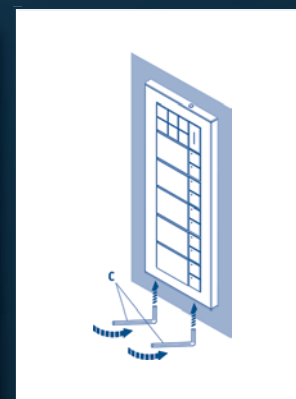
Tighten the Allen screws on the lower part of the surround.
