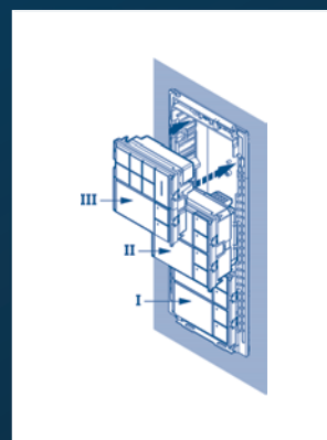
Fit the modules on frame from bottom to top (from I to III).
