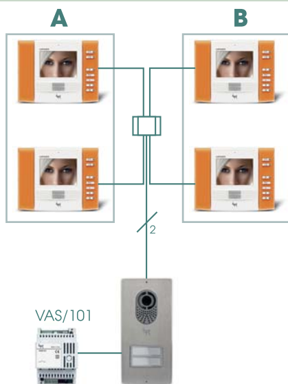
TWO CALLS TO FOUR HANDSETS IN TWO GROUPS
