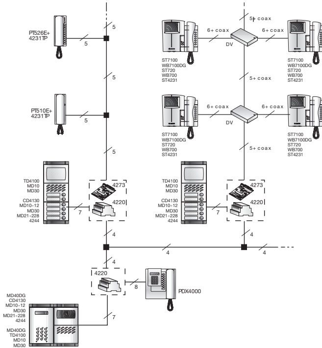
Intercom and video intercom installation with 2 secondary door stations and intercoms with integrated decode module
