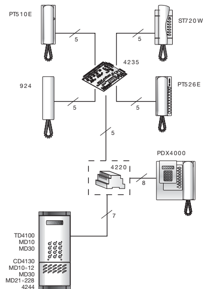
Intercom installation with 1 door station and intercoms with floor decode module
