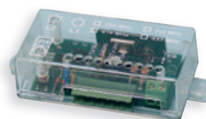
RX26-433I/RX39-433 (2 channel) 105 x 45 x 28mm
