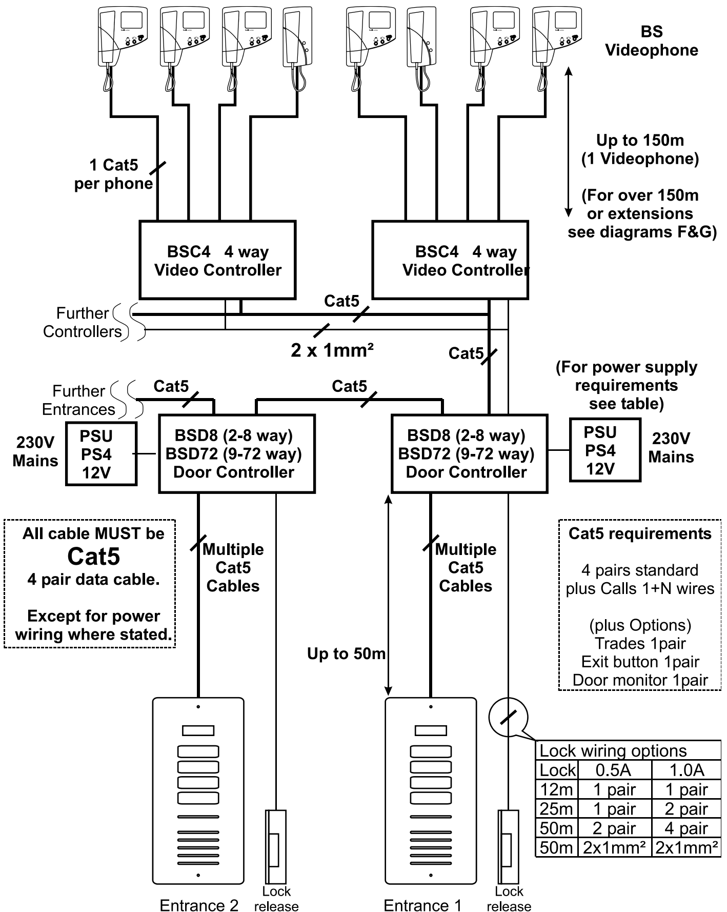
Diagram A – 2-72 Way Basic System Overview Cabling
