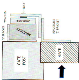
BKEX1200ZL Inward Opening
