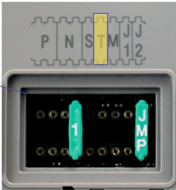
Jumpers in slots J1 and J2 may vary depending on kit used, please see p. 3 for required configuration details
