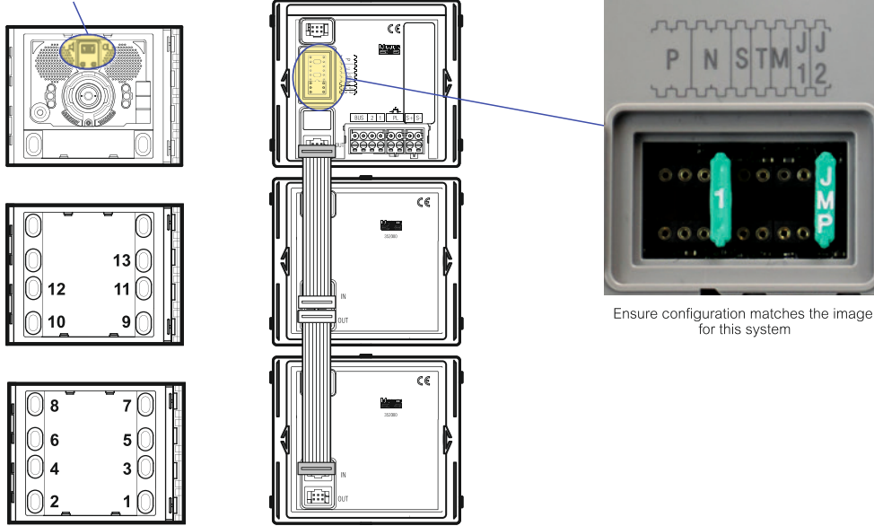
Push button layout
