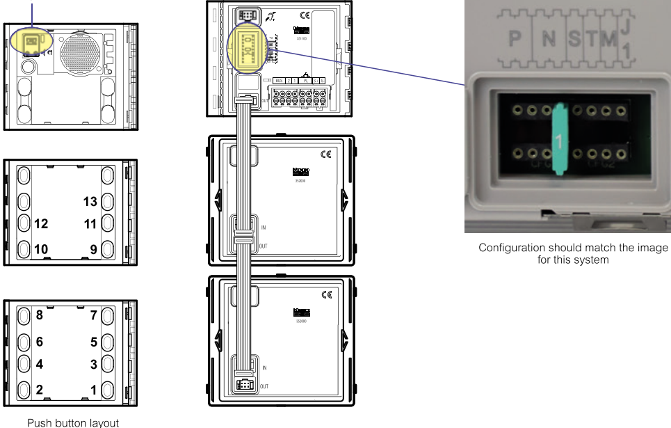
Push button layout
