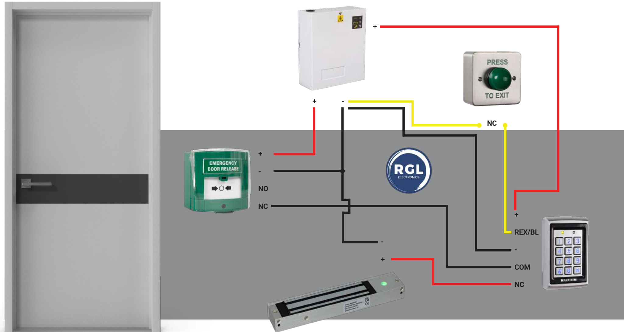
wiring diagram
