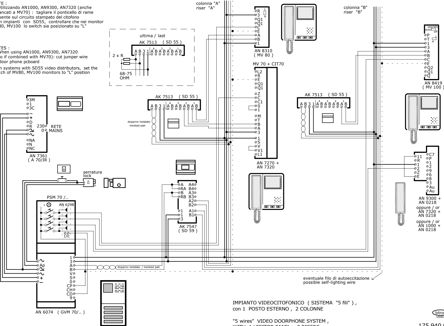
"5 wires" VIDEO DOORPHONE SYSTEM , WITH 1 VISITOR PANEL, 2 RISERS
