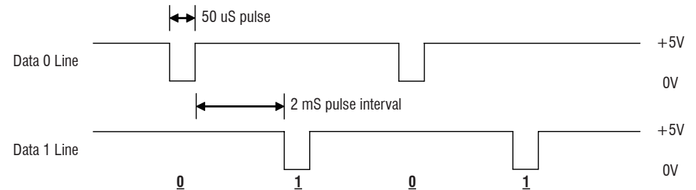
Diagram of The Wiegand Protocol Timing and Its Electrical Manner
